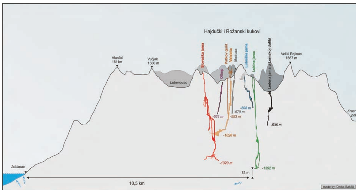
Fig. 30: Cross-section through Velebit mountain with outstanding caves (published with permission of the author-D. Bakšić).
