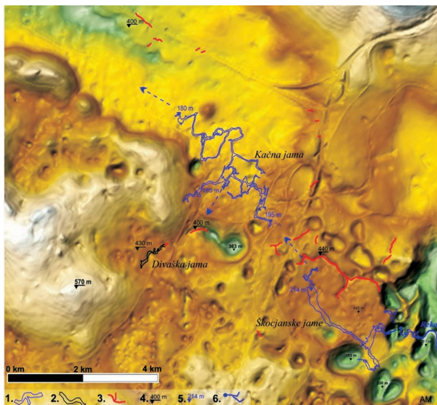
Fig. 29: Divača karst is the best Dinaric example of the interrelation between contact karst features - ponor caves, collapse dolines and unroofed caves (DEM source: ASTER GDEM 1"; figure made by: A. Mihevc).
